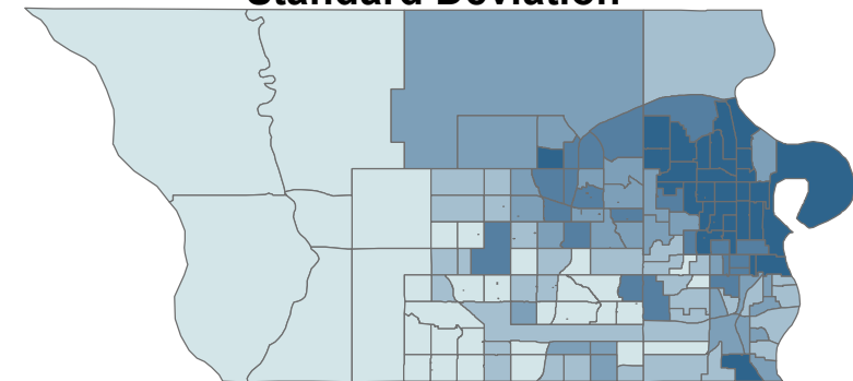
Standard Deviation
