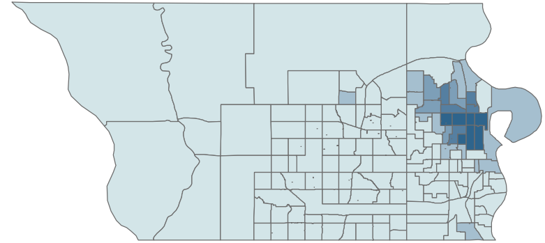
Natural Breaks
