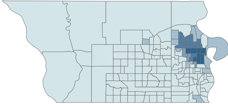
Equal Interval
