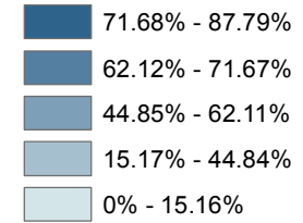
Standard Deviation
